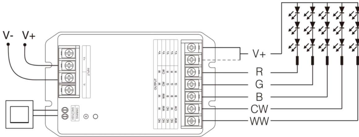
PUSH switch
