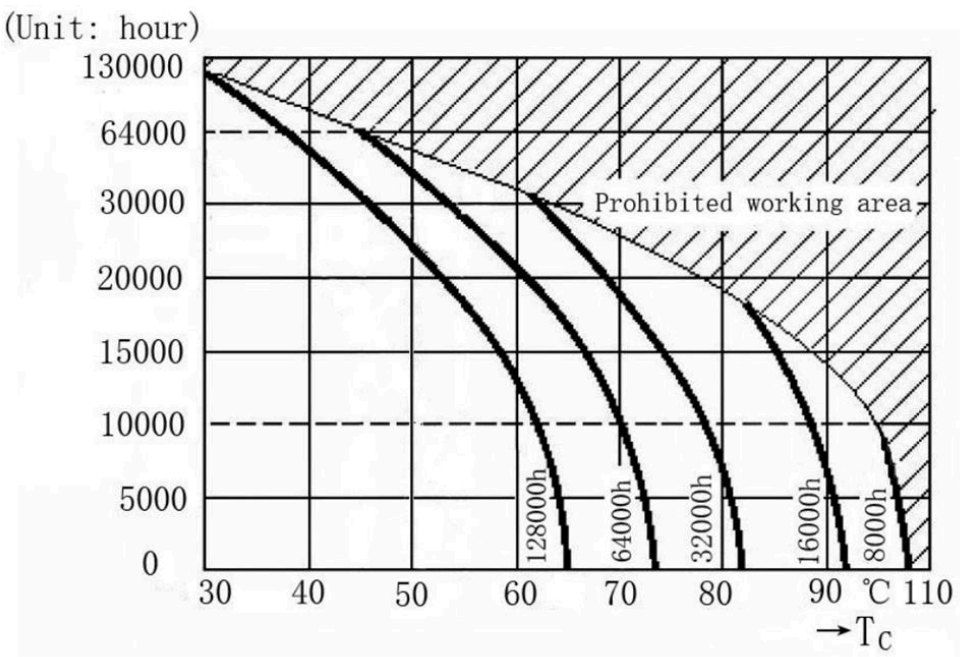
Power supply operating temperature and life curve
